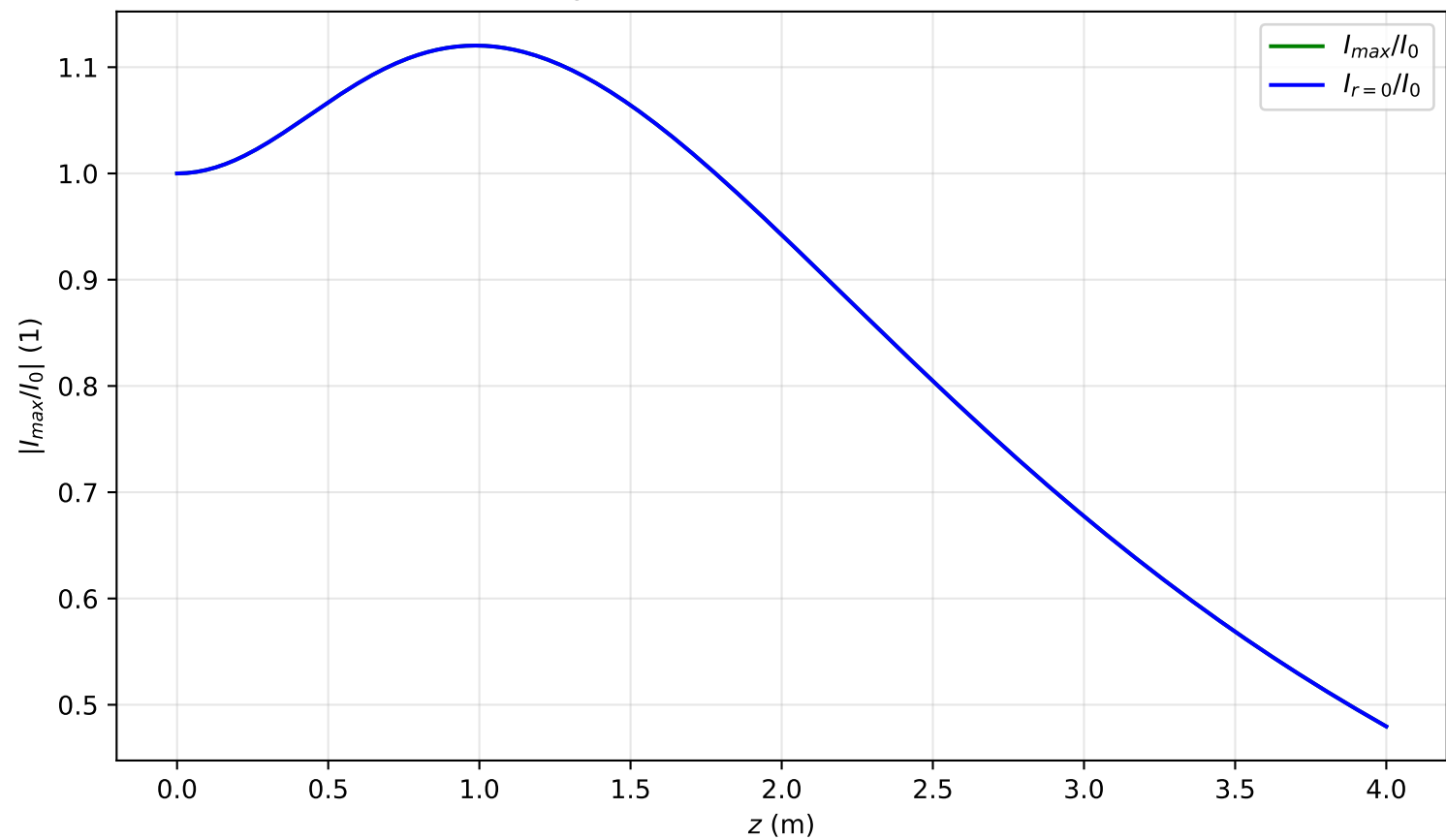
I_{max}(x = 0, y = 0, z)/I_0 , P_{in}=0.6P_{cr} , artificial time
